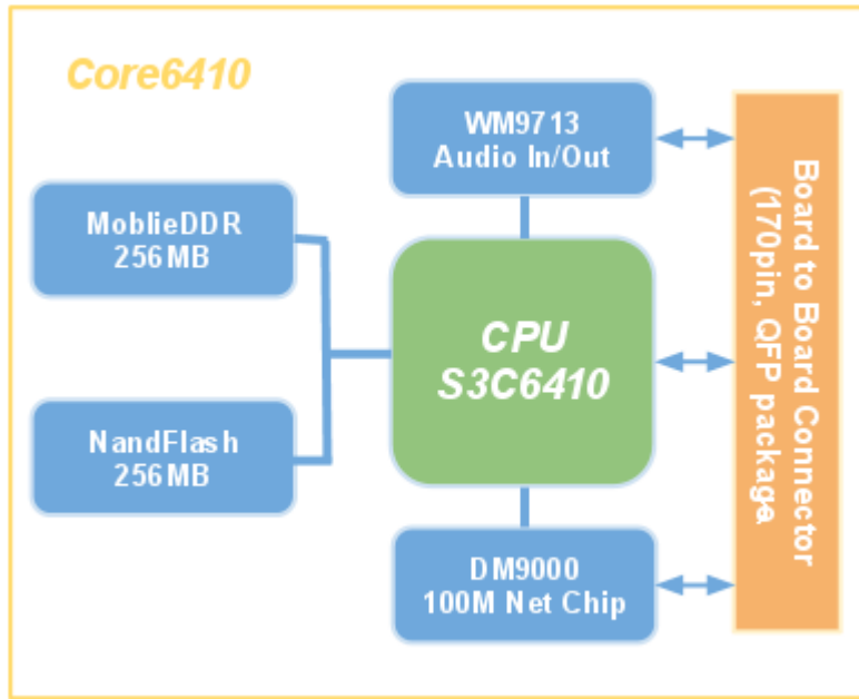
CoreWind Core6410 Functional Block Diagram
